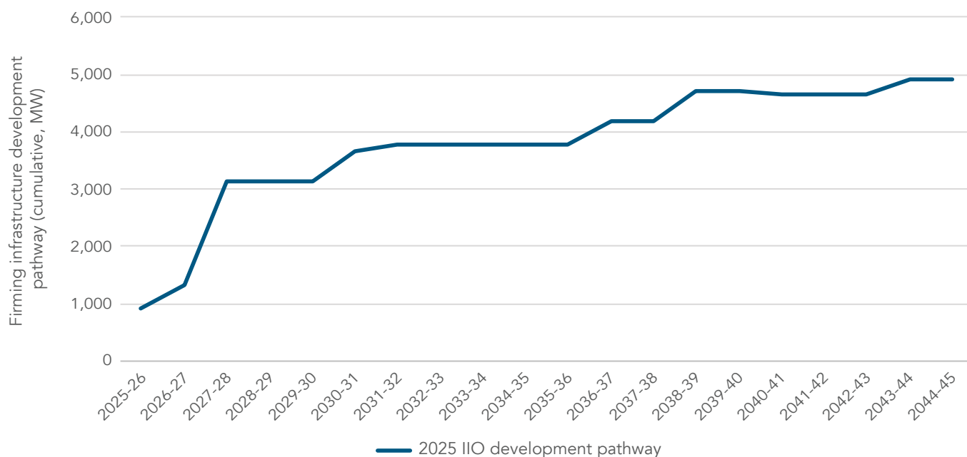
Figure 5: Firming infrastructure element of the development pathway
