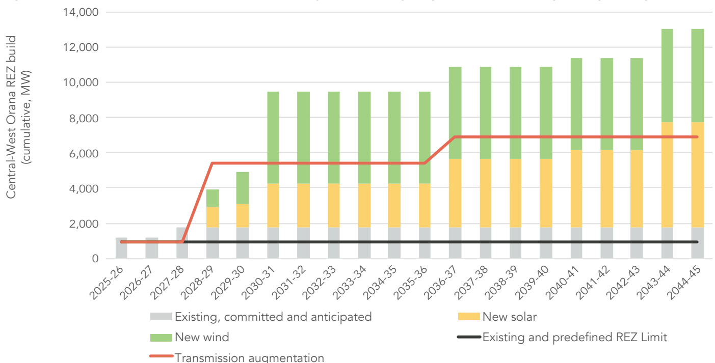
Figure 26: Central-West Orana REZ network and generation capacity under the development pathway
